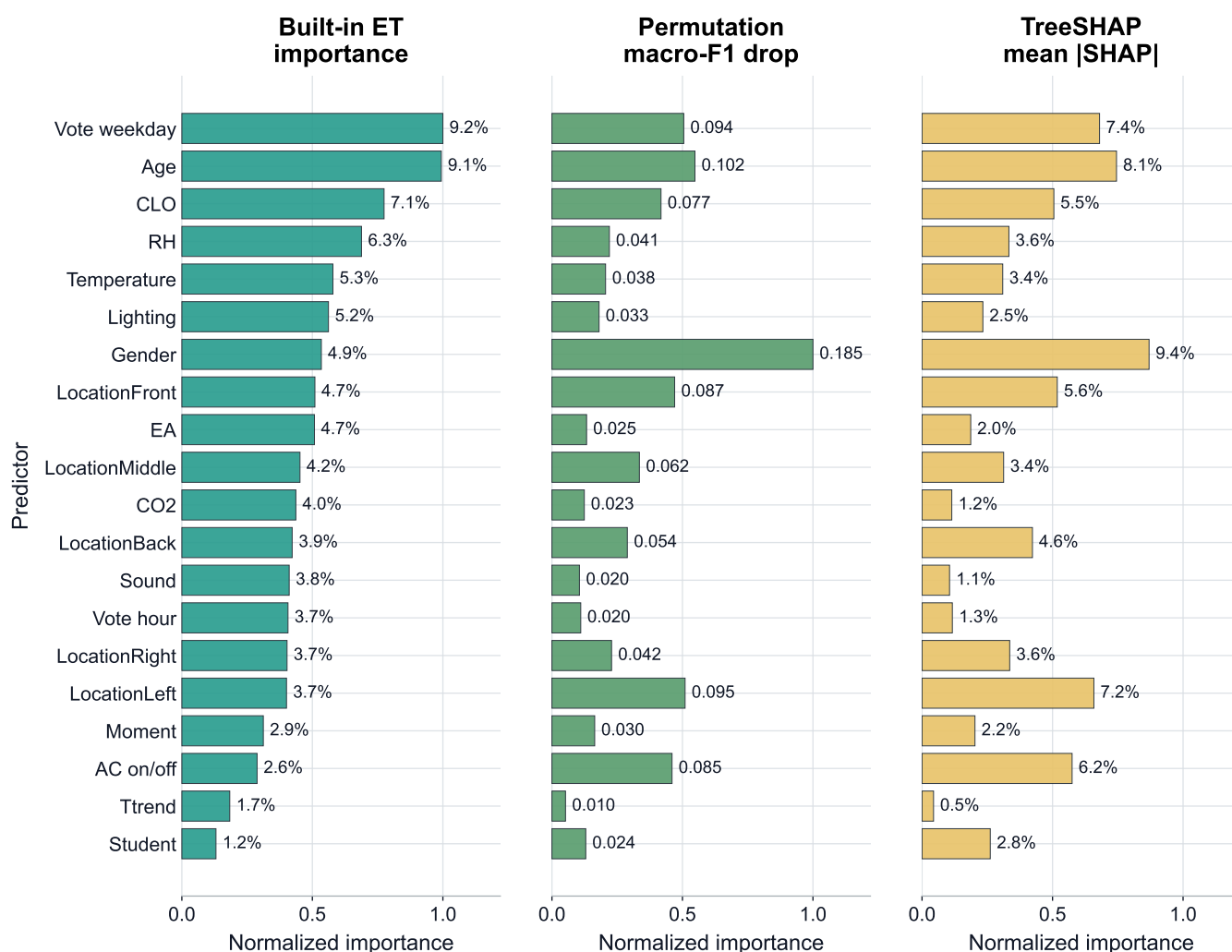
Figure 10: Feature-importance comparison for the final Extra Trees IEQ prediction model. All original predictors are shown; imputation indicators are excluded.
