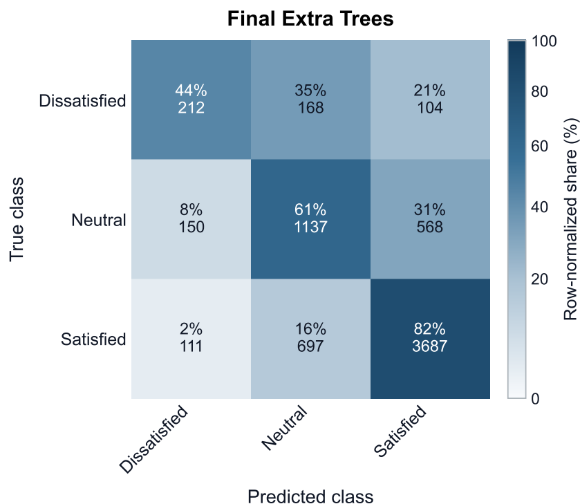
Figure 9: Out-of-fold confusion matrix for the final Extra Trees model. Cells show row percentages and counts.
