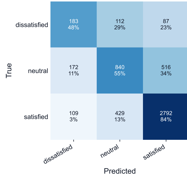
5-class collapsed to 3-class
