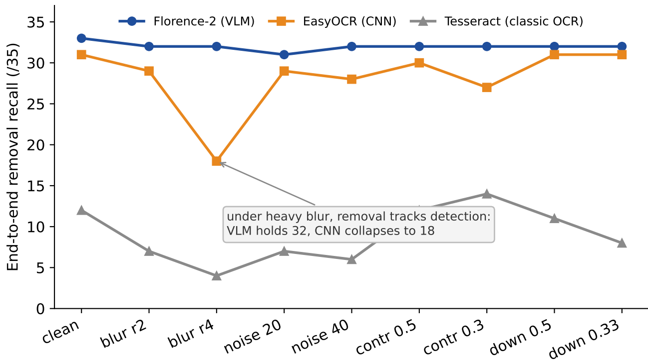
End-to-end PHI removal under degradation (full pipeline, strict)
