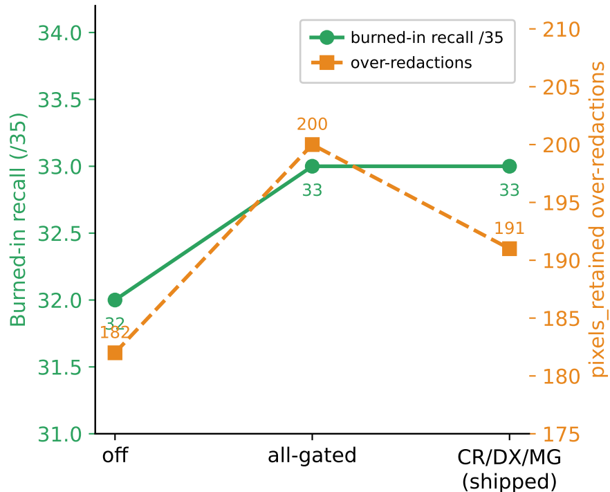
(b) Margin rule: recall vs precision
