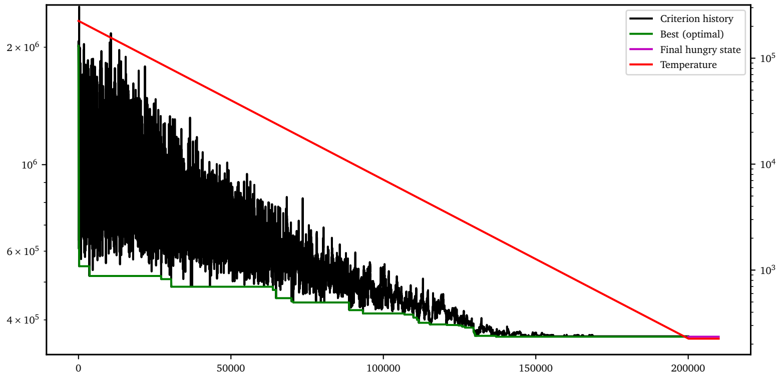
Progress of Simulated Annealing combinatorial optimization
