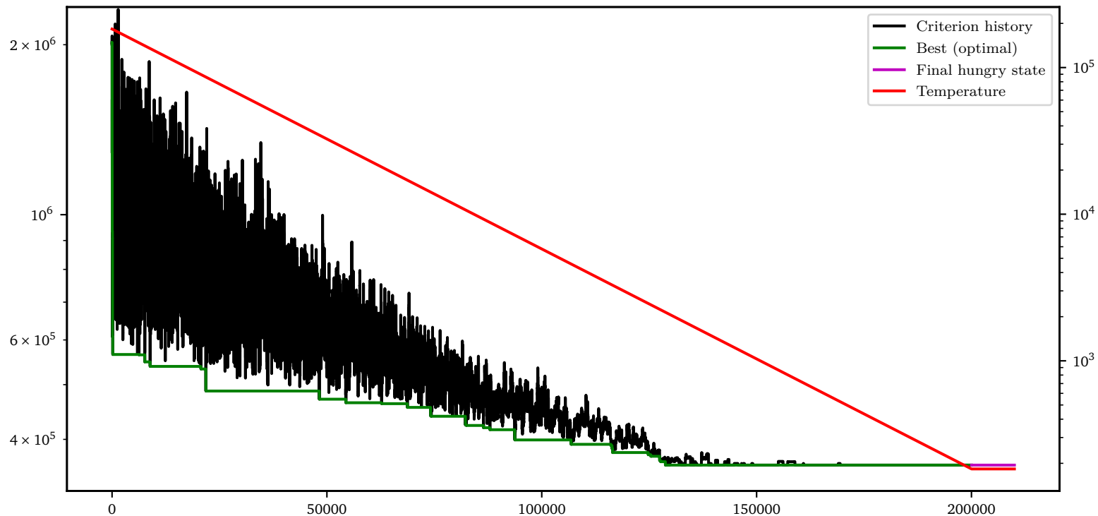
Progress of Simulated Annealing combinatorial optimization
