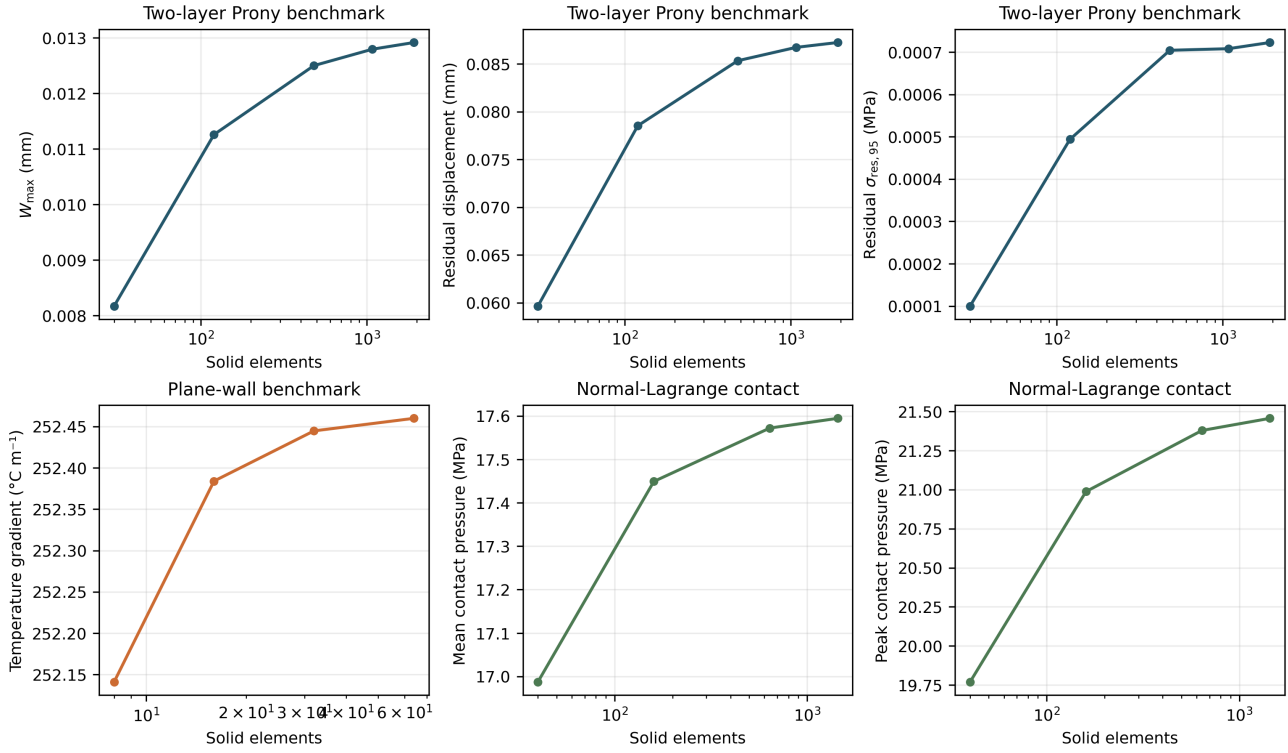
Figure 2. Mesh refinement for genuine MAPDL verification configurations. The structural, thermal and contact values are numerical-fixture responses; they are not production PLA annealing predictions. Every plotted point is linked to an archived solver run.
