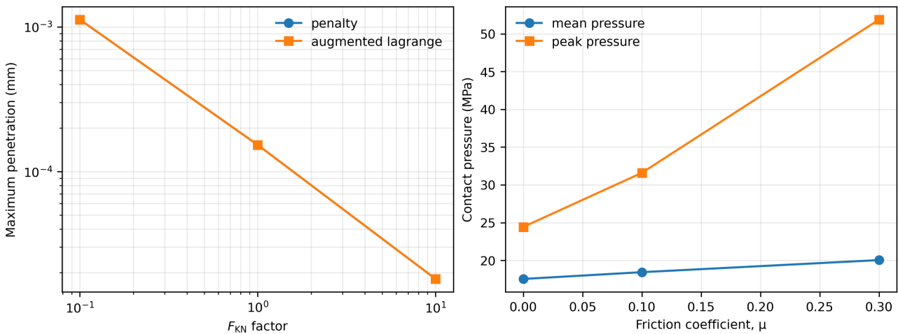
Figure 4. Contact-control responses in the numerical fixture. Penalty stiffness and friction are declared perturbations rather than sourced production interface parameters. Algorithm differences must be retained when comparing cases.
