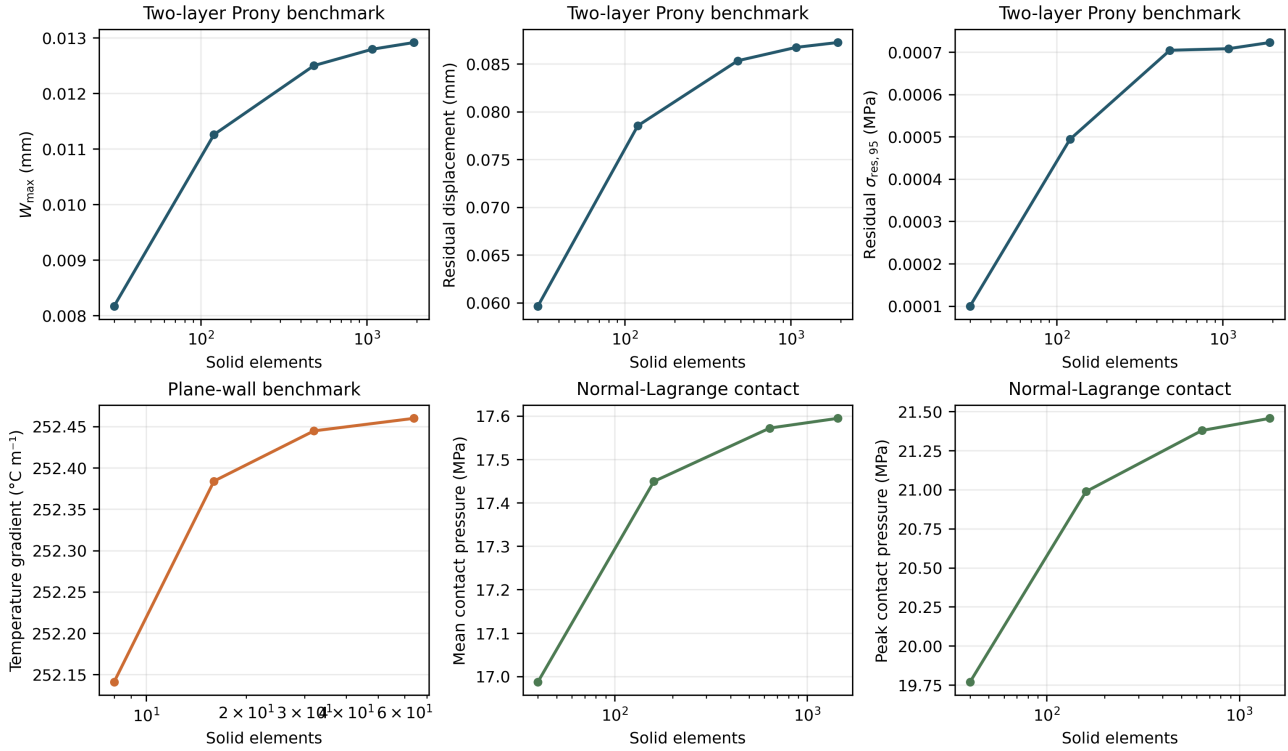
Figure 2. Genuine MAPDL mesh-refinement responses for numerical structural, thermal and surface-contact configurations. Every point traces to an archived solver run; no point is a production annealing prediction.
