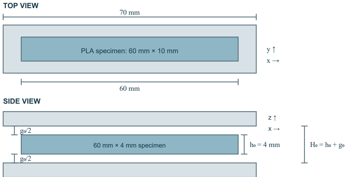
Figure 1. Candidate coupon and opposed-plate geometry at the reference state. The schematic contains no solved mesh, temperature, contact or deformation field.
