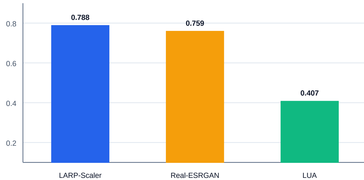
Photo — SSIM ↑
