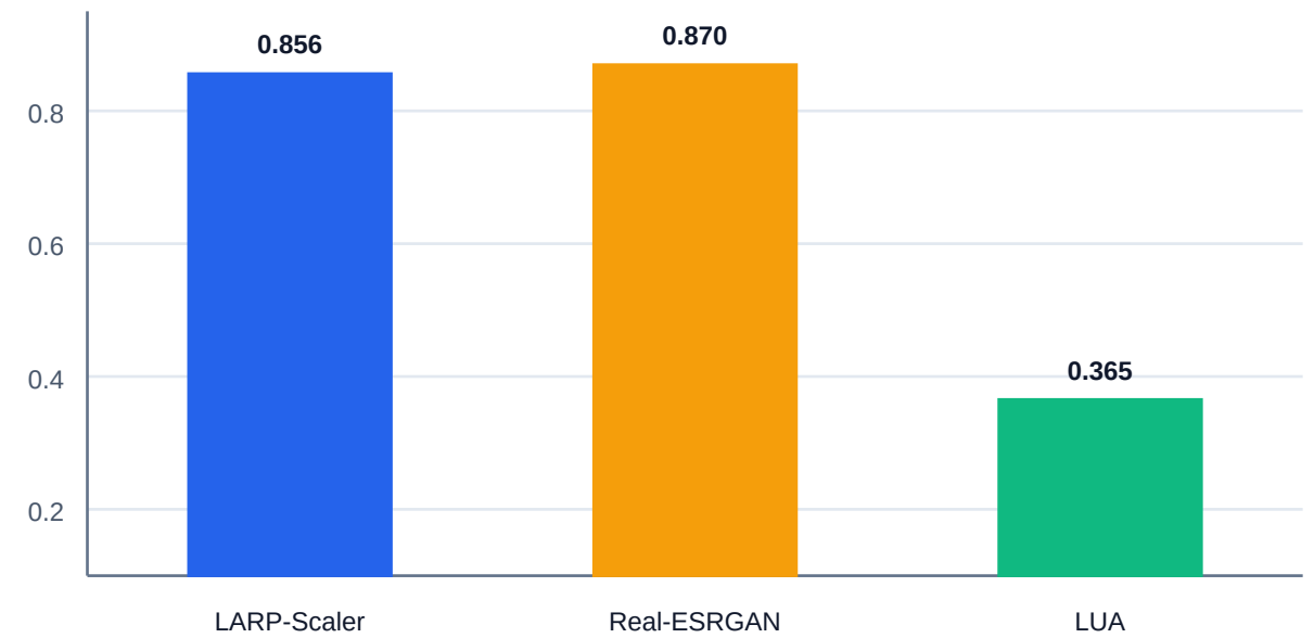
Anime — SSIM ↑
