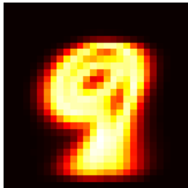
\hat{\Sigma}_9 (diag.)
