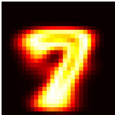
\hat{\Sigma}_7 (diag.)
