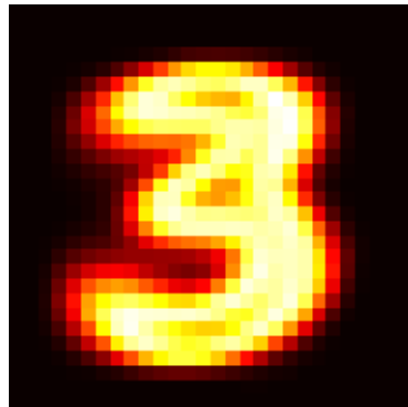
\hat{\Sigma}_8 (diag.)
