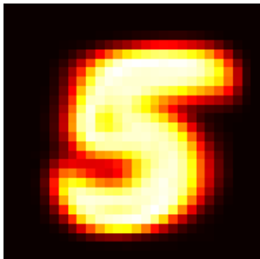
\hat{\Sigma}_5 (diag.)
