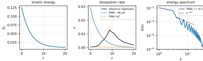
Figure 2: Benchmark D: kinetic energy, the two dissipation estimates of the network against the digitised reference [33], and the spectrum at t = 9 .
