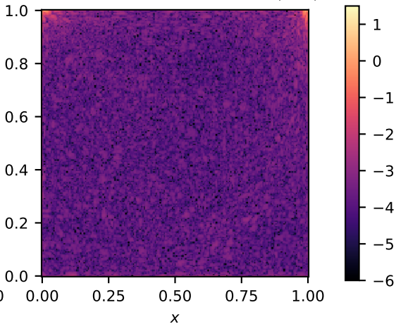
row C, soft boundary data: \log_{10} |\nabla \cdot u|
