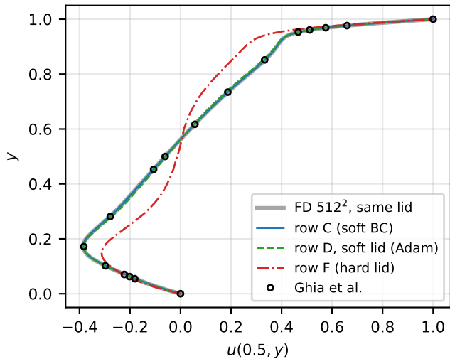
vertical centreline, Re = 1000
