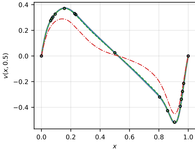
horizontal centreline, Re = 1000
