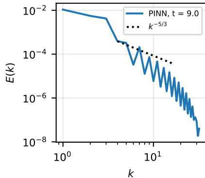
energy spectrum
