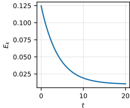
kinetic energy
