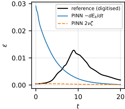
dissipation rate
