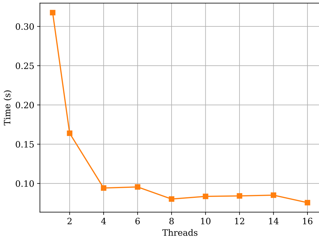
Execution Time - B
