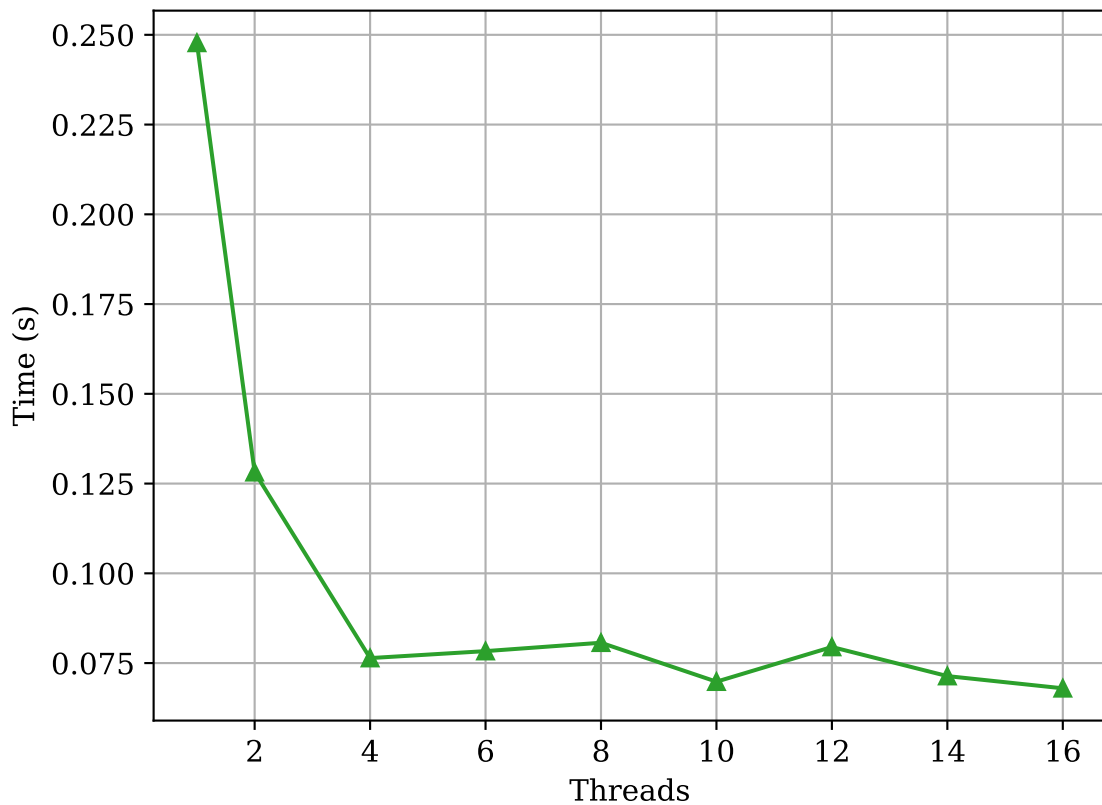
Execution Time - C
