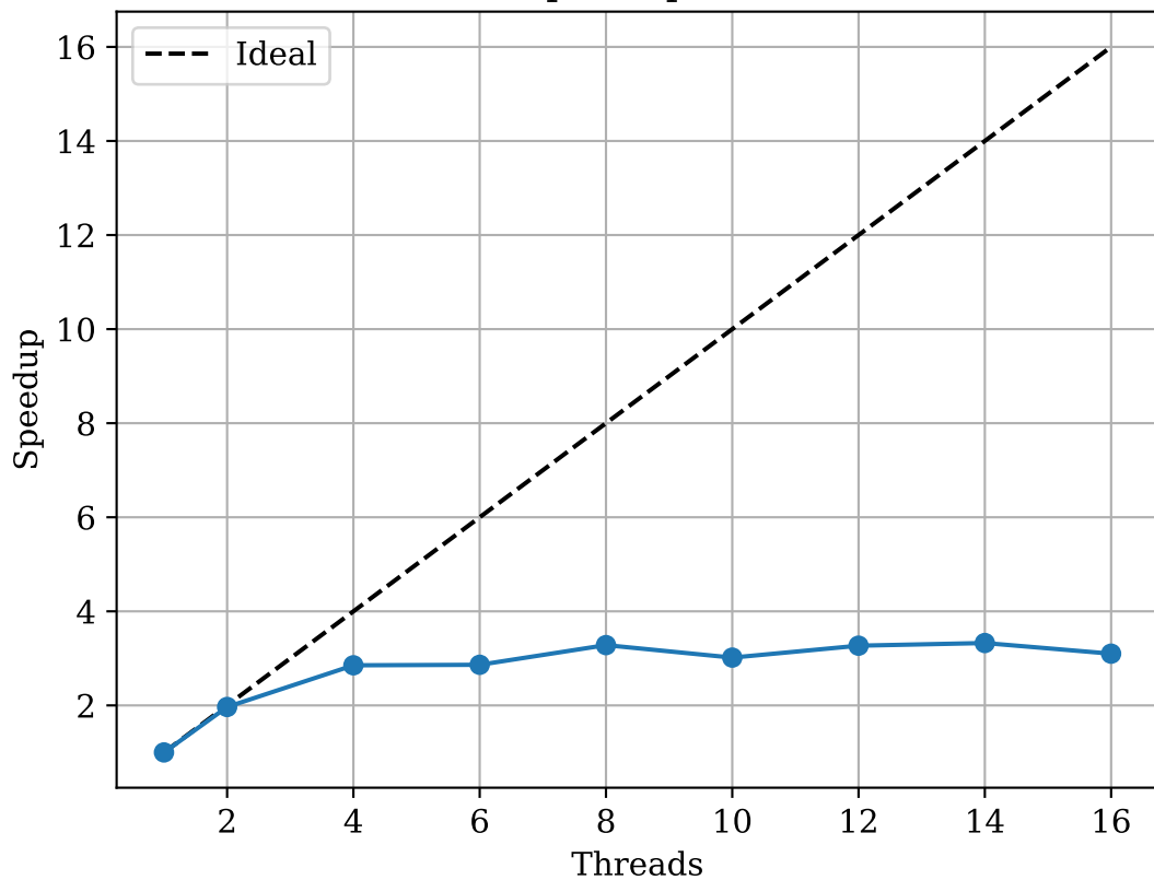
Speedup - A
