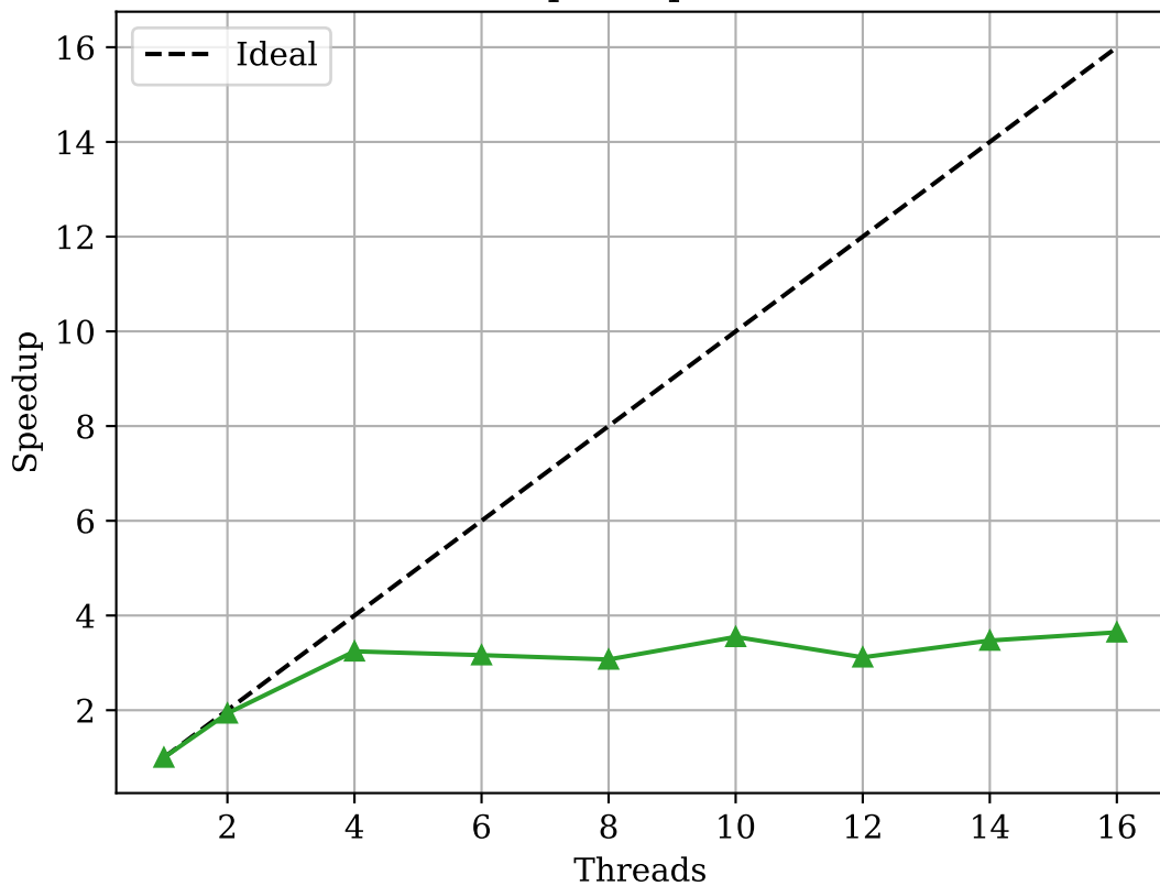
Speedup - C
