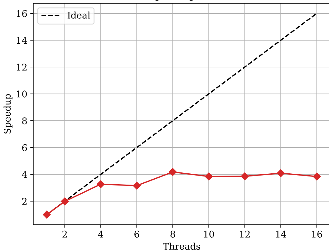
Speedup - D
