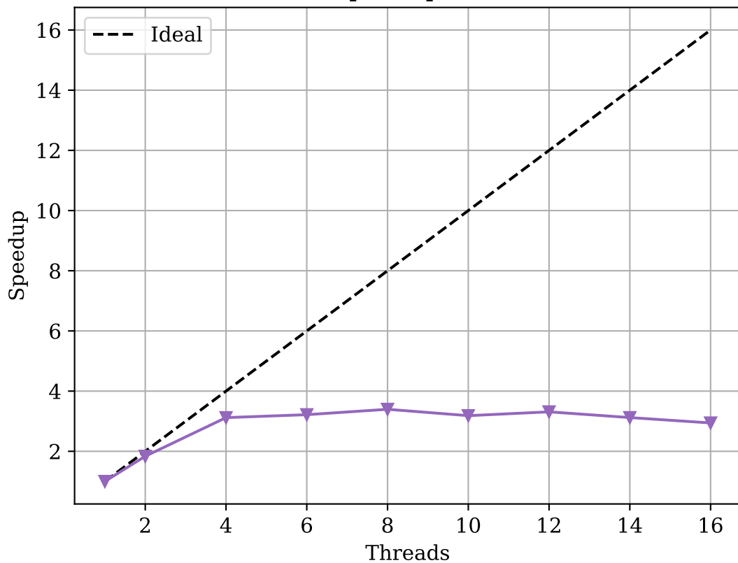
Speedup - E
