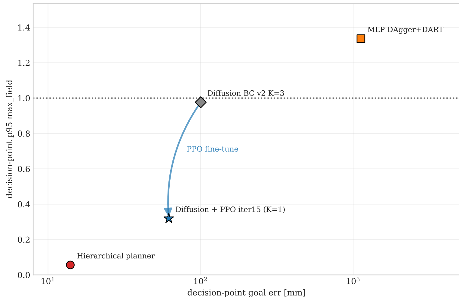
Decision-point safety vs goal-reaching
