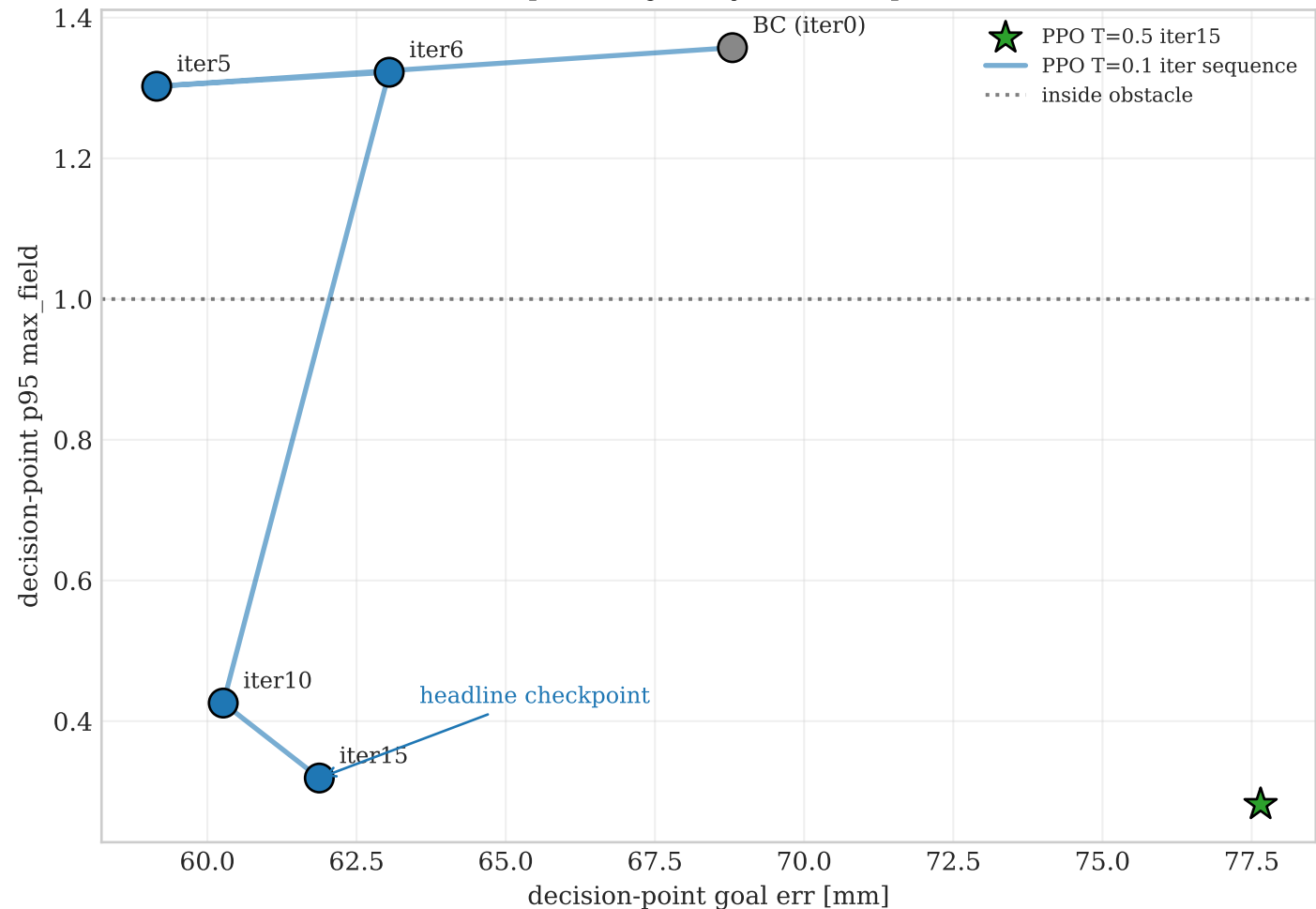
PPO checkpoint trajectory (decision-point eval)
