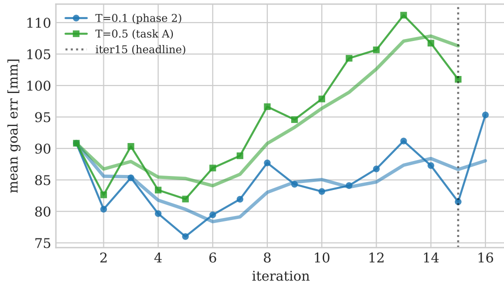
Goal-reaching per iter
