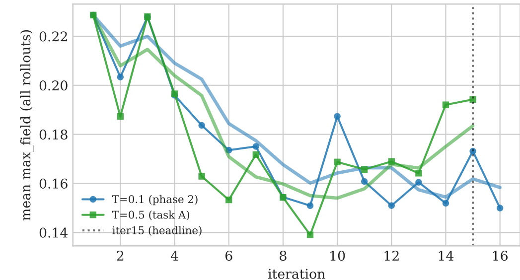
Safety -- mean max_field per iter
