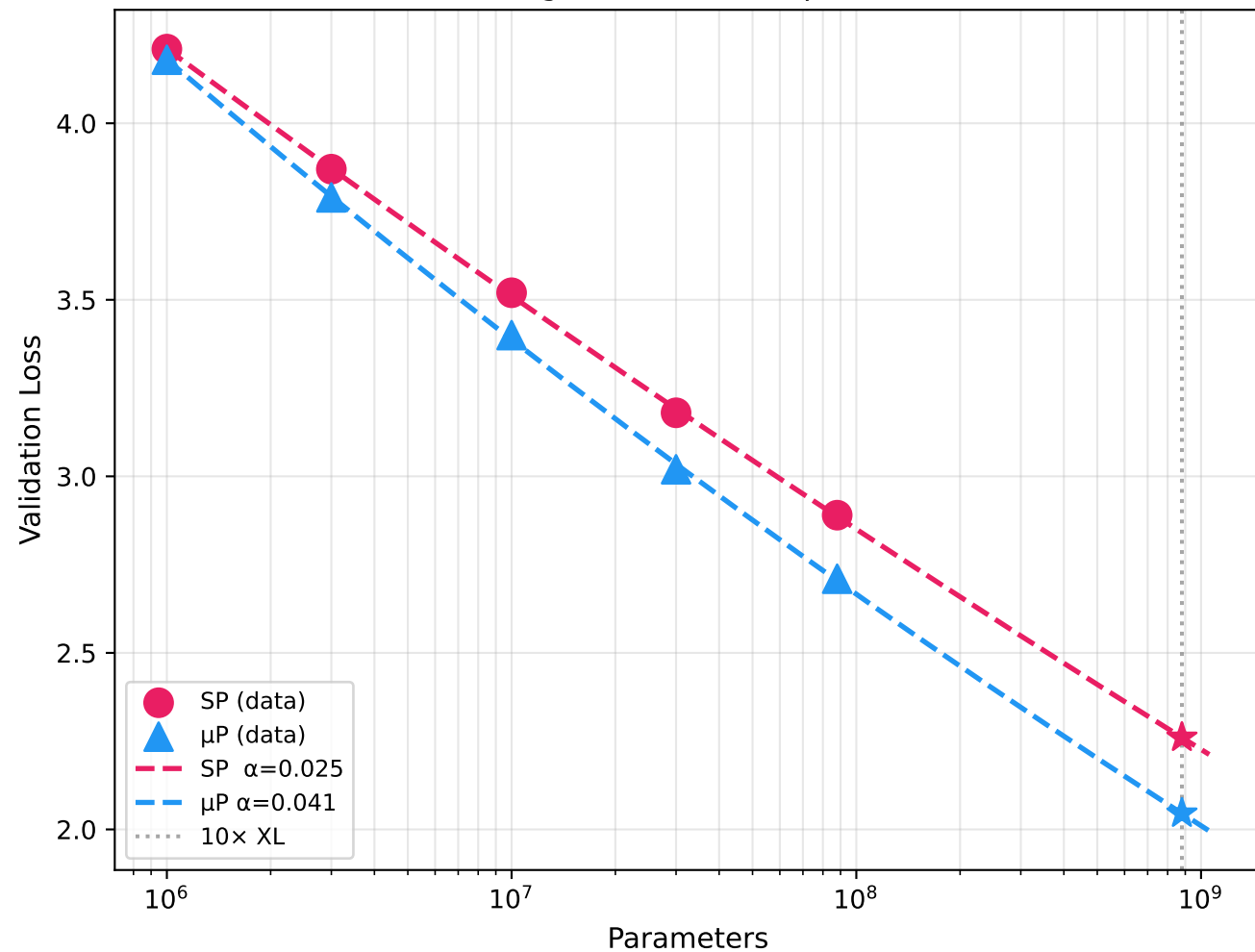
Scaling Curves + Extrapolation
