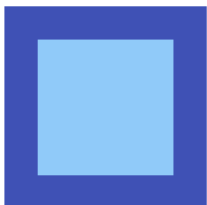
Prefix 3 (Group+rect)
