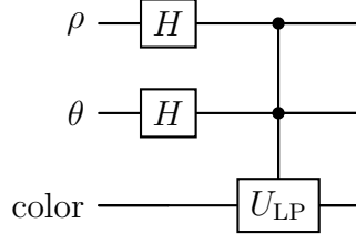
Figure 11: QLR circuit with log-polar coordinate encoding.
