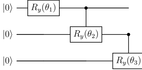
Figure 10: QPIE circuit using probability amplitude encoding.
