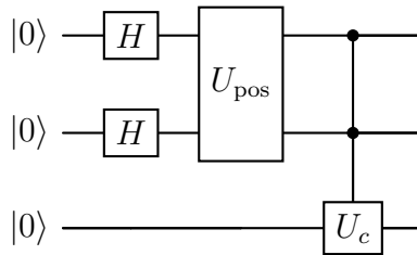
Figure 4: GQIR circuit with generalized position encoding U_{\text{pos}} for arbitrary image dimensions.
