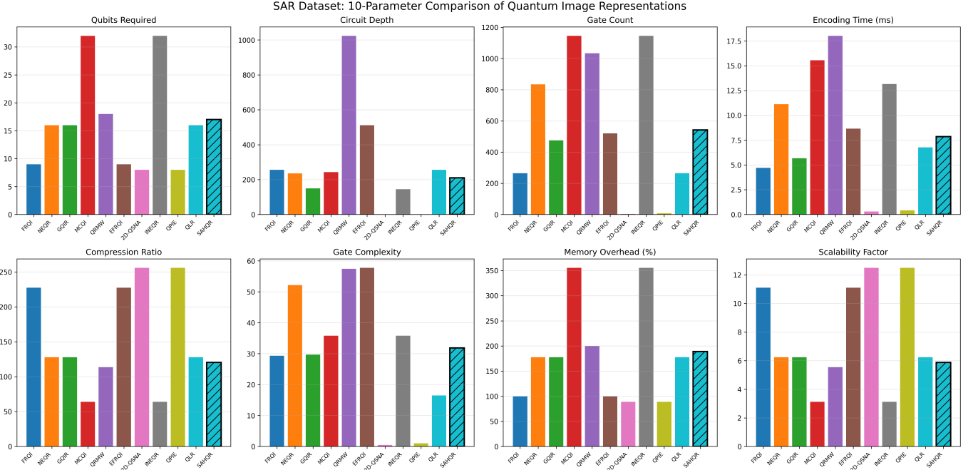
Figure 24: SAR Dataset: 10-parameter comparison of quantum image representation methods across 2,000 satellite imagery tiles. SAHQR (hatched bars) demonstrates balanced performance across all evaluation metrics.
