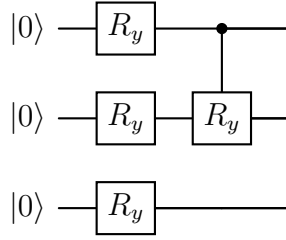
Figure 8: 2D-QSNA circuit using amplitude encoding with rotation gates.
