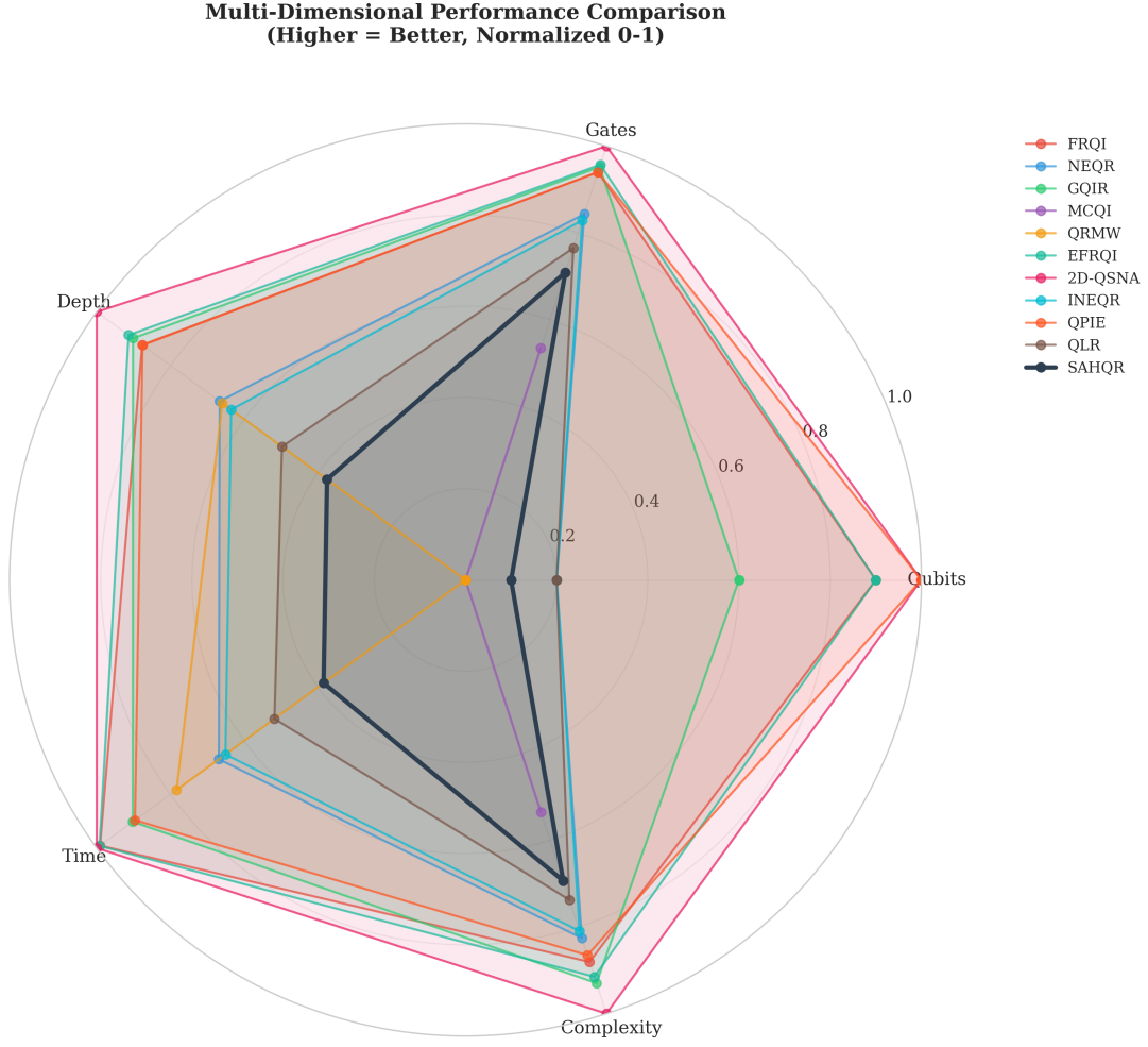
Figure 17: Multi-dimensional performance comparison using a radar plot. Each axis represents a normalized performance metric (higher is better). SAHQR (black line) achieves balanced performance across dimensions.
