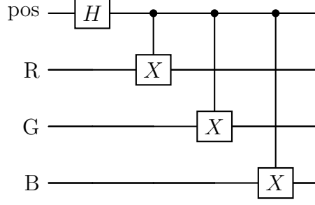
Figure 9: INEQR circuit with improved color channel encoding.
