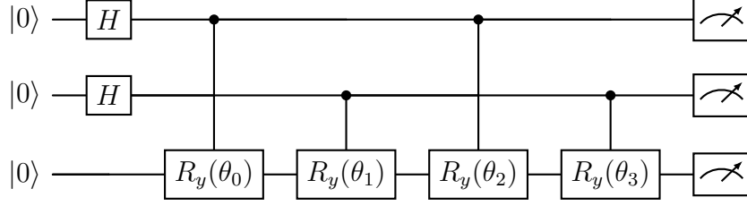
Figure 2: Simplified FRQI circuit for a 2 \times 2 image. Position qubits (top two) control rotation gates applied to the color qubit (bottom).
