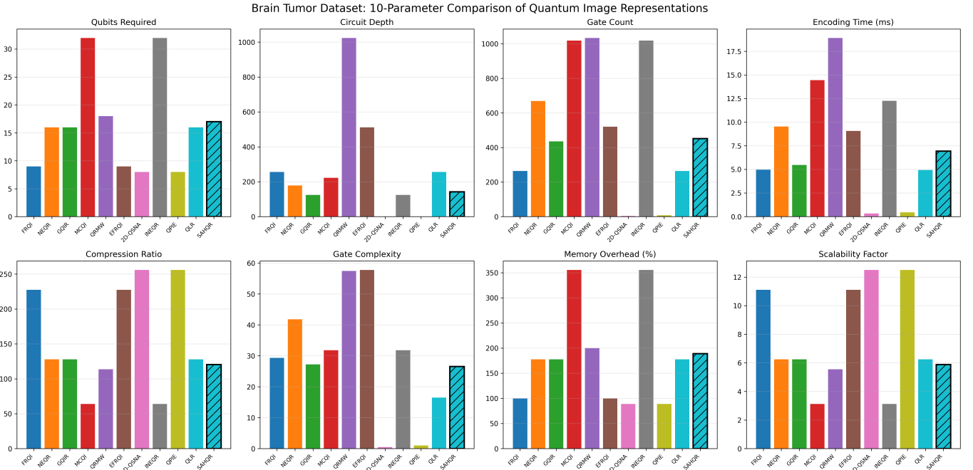
Figure 25: Brain Tumor Dataset: 10-parameter comparison of quantum image representation methods across 2,298 MRI scans. SAHQR (hatched bars) maintains consistent performance characteristics observed in other domains.
