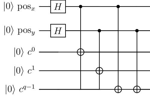
Figure 3: Simplified NEQR circuit structure. Position qubits control CNOT gates that set color qubit values.
