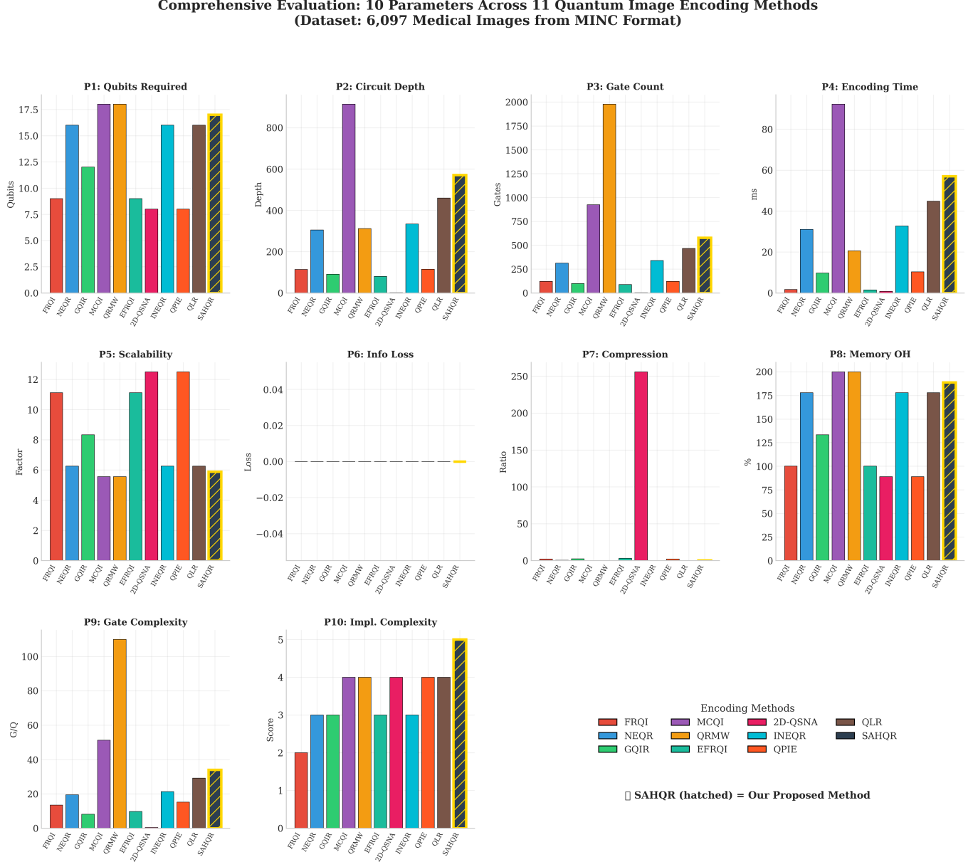
Figure 16: Comprehensive evaluation of 10 parameters across 11 quantum image encoding methods. SAHQR (hatched bars) demonstrates competitive performance across most metrics while uniquely providing content-aware encoding capability.
