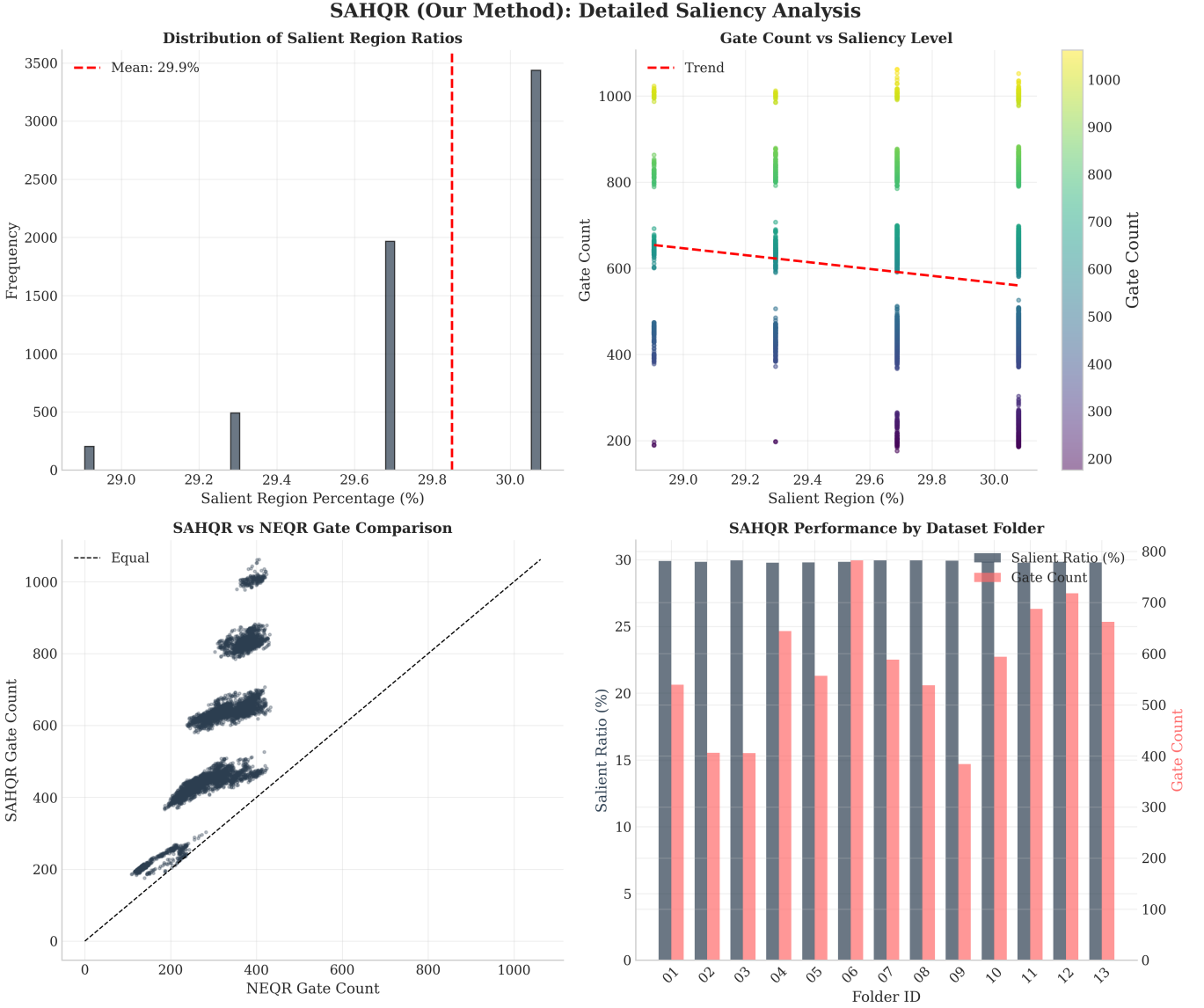
Figure 19: SAHQR detailed saliency analysis. (a) Distribution of salient region ratios across dataset. (b) Gate count vs. saliency level correlation. (c) SAHQR vs. NEQR gate comparison showing reduction in non-salient regions. (d) Performance variation across dataset folders.
