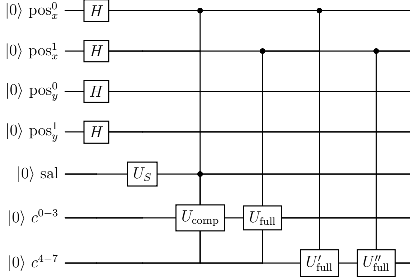
Figure 13: SAHQR circuit architecture. Position qubits (pos) encode pixel locations. The saliency qubit (sal) controls differential encoding: U_{\text{comp}} for non-salient, U_{\text{full}} for salient regions. Color qubits ( c^{0-7} ) store pixel values.
