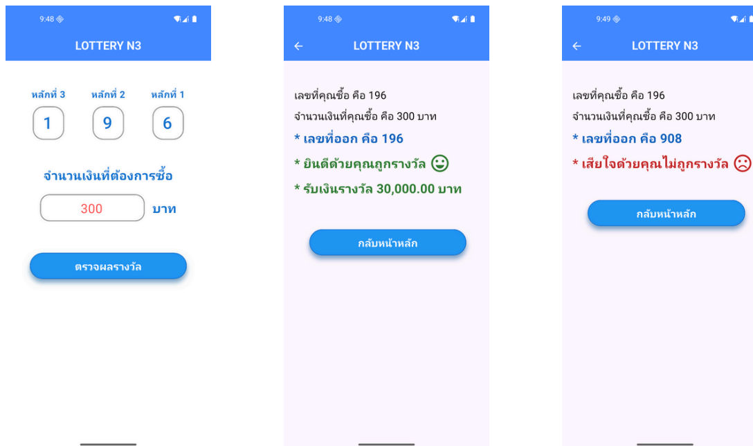
App: Lottery file : main.dart
