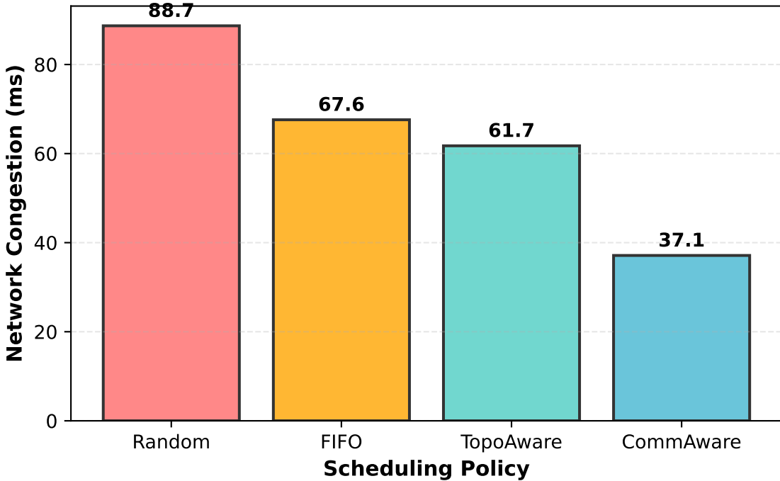
Network Congestion by Scheduling Policy
