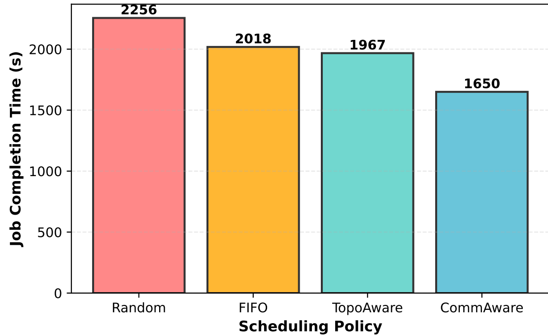
Average Job Completion Time by Policy
