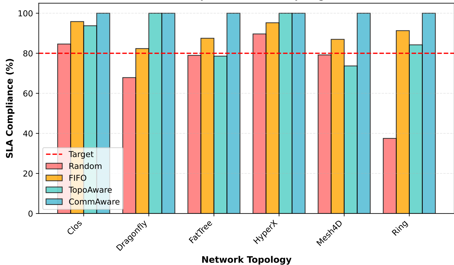
SLA Compliance Across Topologies
