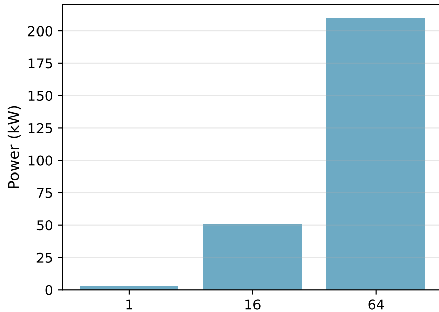
BERT-base
