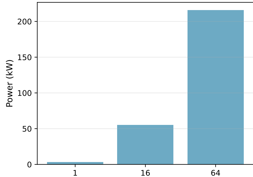
CosmoFlow
