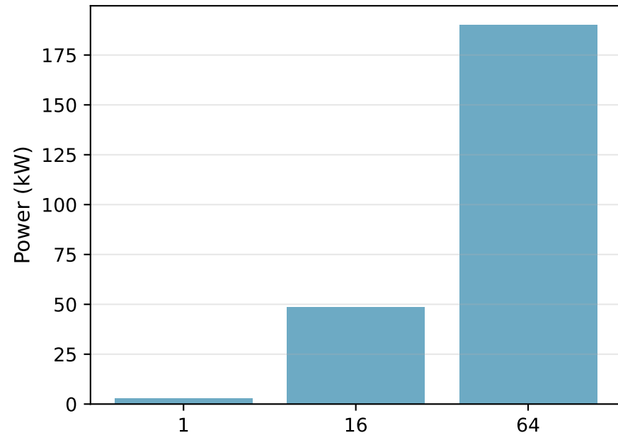
ResNet-50
