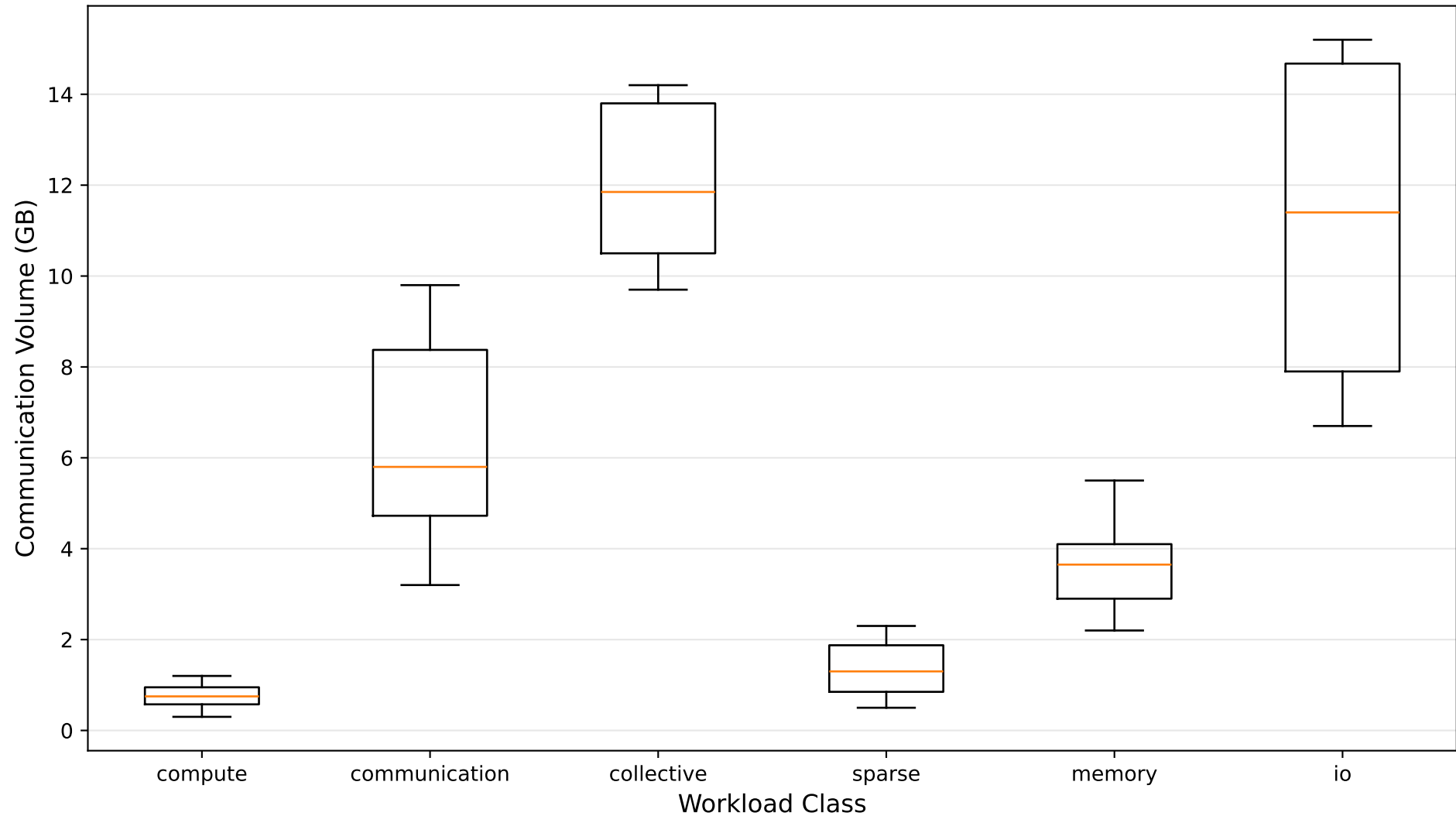
Network Demand Distribution by Workload Class
