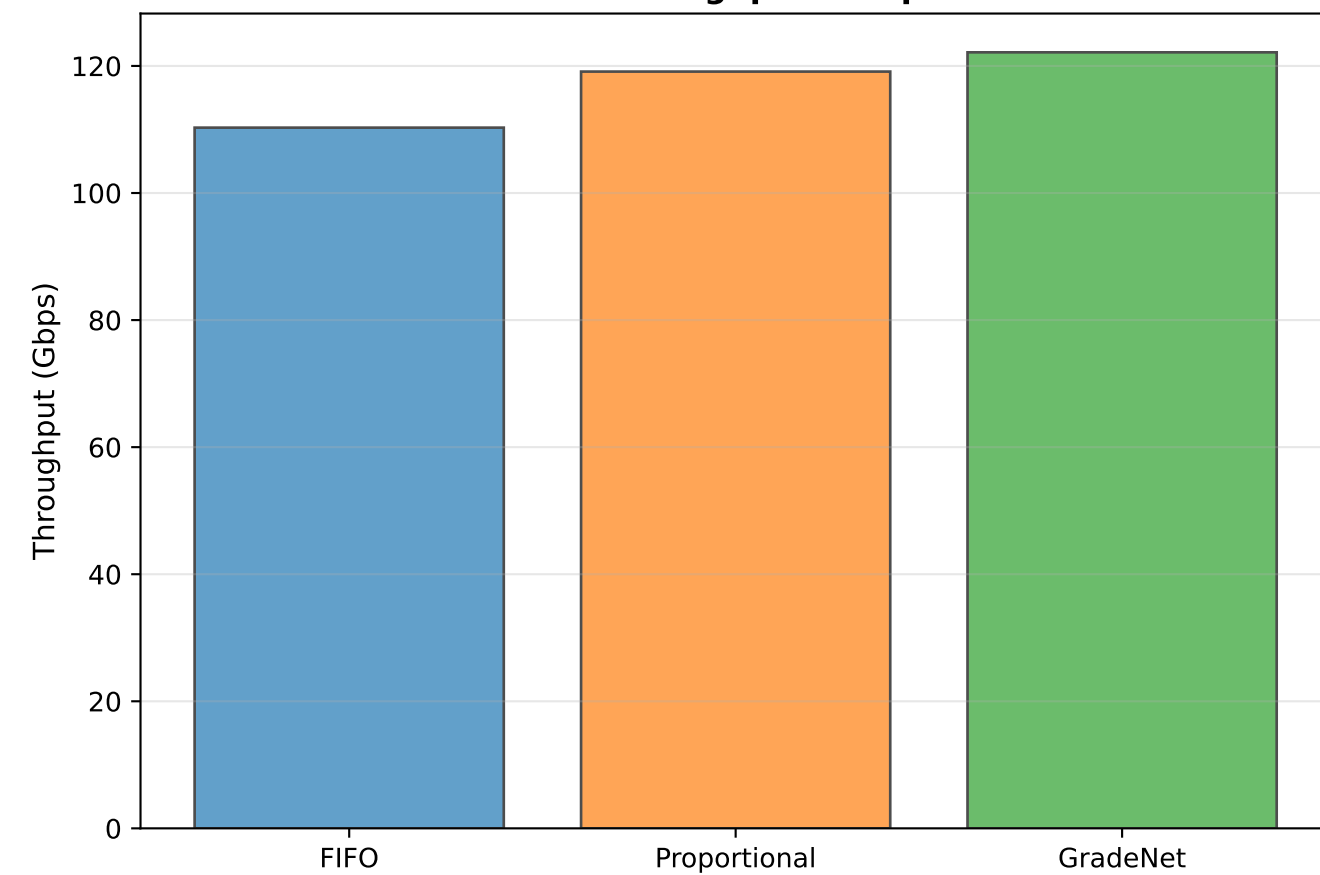
GradeNet Performance Improvements
