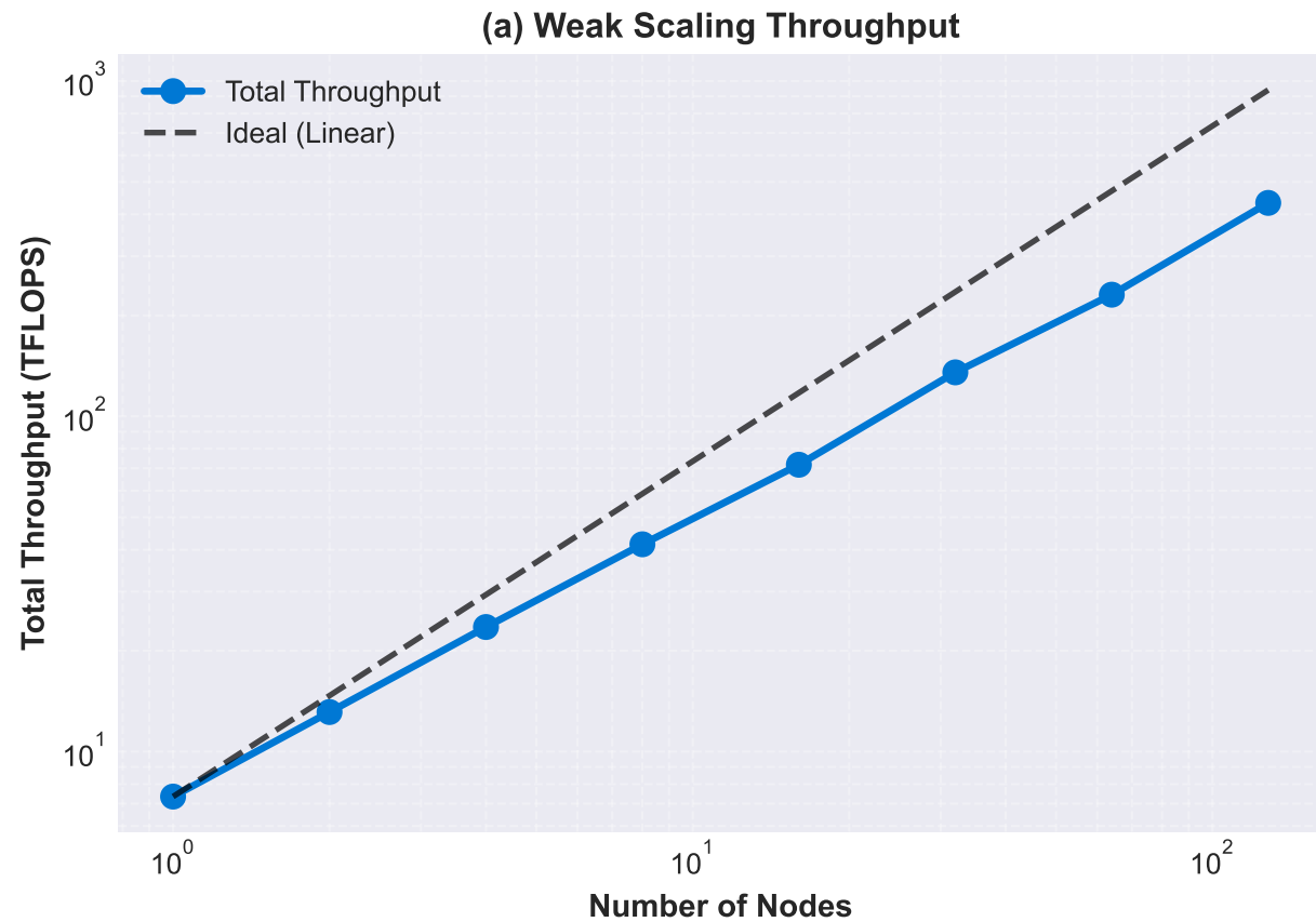
Figure 5: Weak Scaling Analysis (Proportional Workload Increase)
