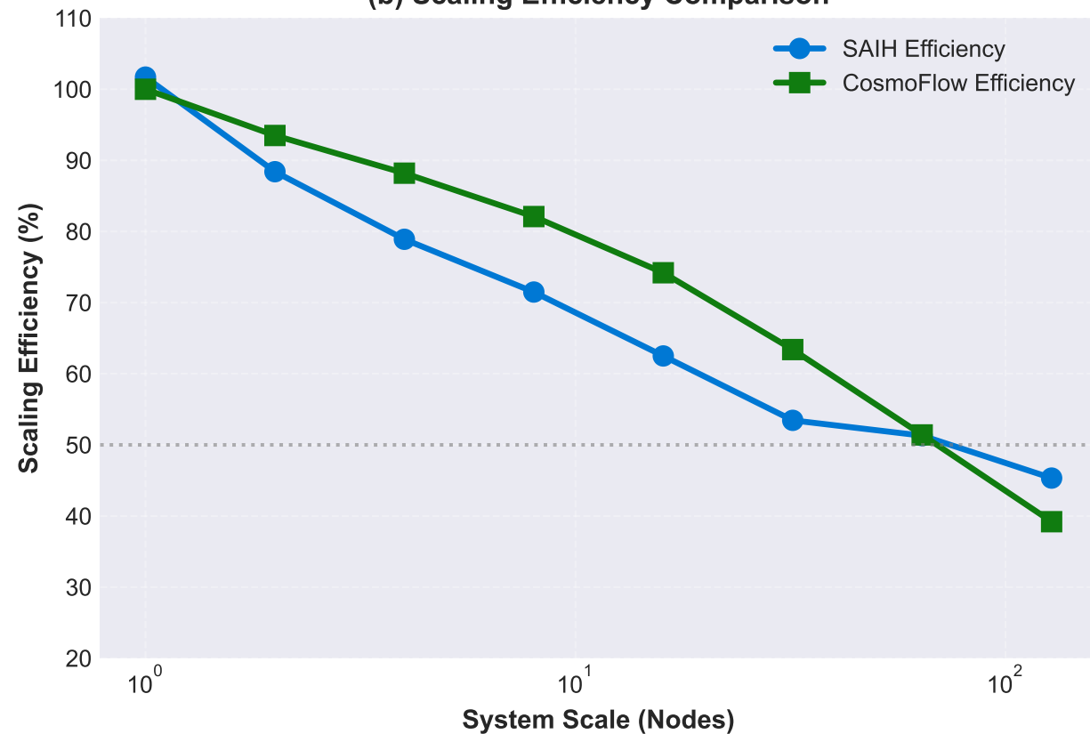
(b) Scaling Efficiency Comparison
