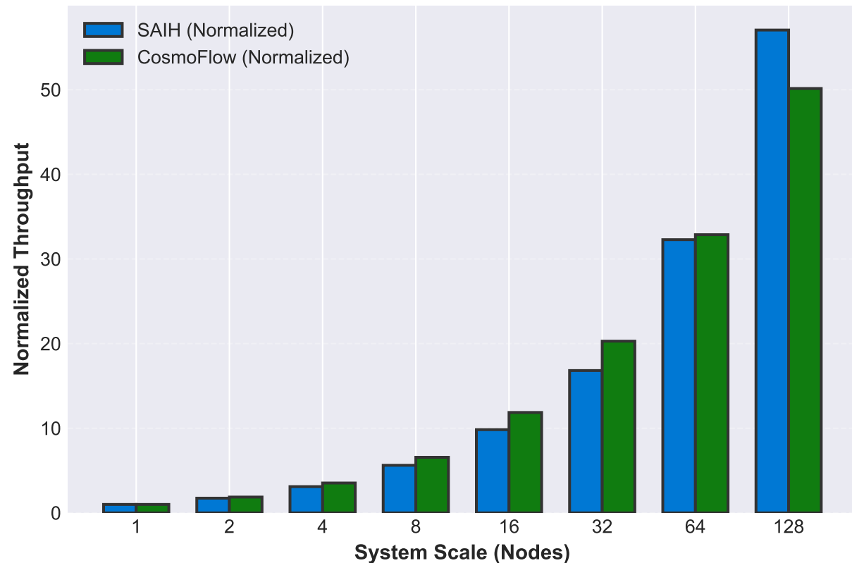
(a) SAIH vs MLPerf-HPC Scaling Trends
