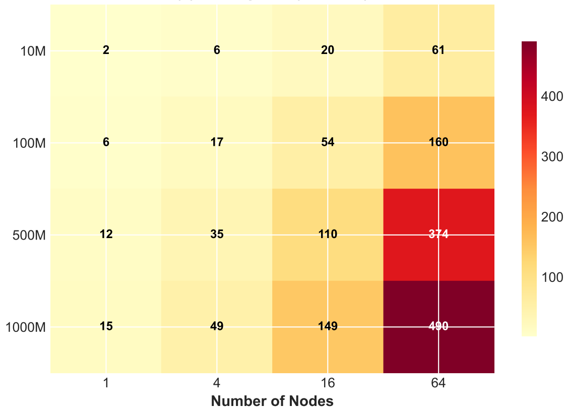
(a) Throughput (TFLOPS)
