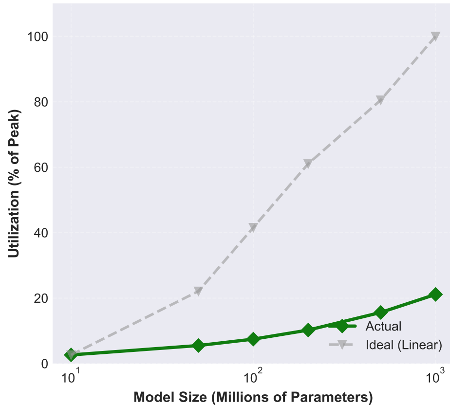
(b) Utilization vs. Model Complexity
