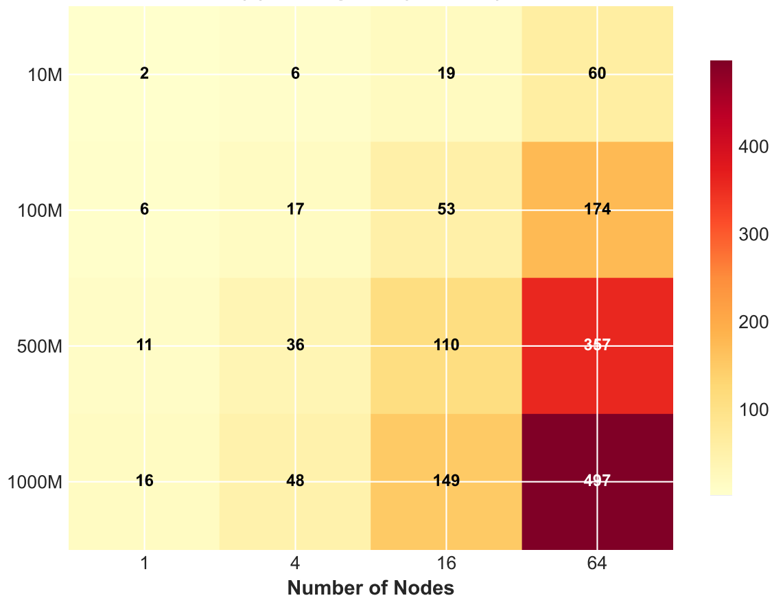
(a) Throughput (TFLOPS)
