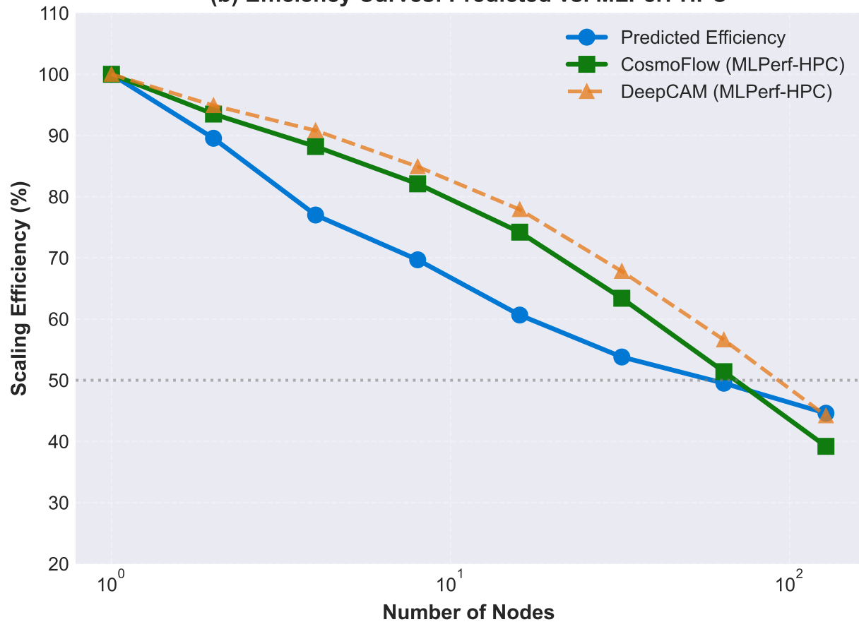
(b) Efficiency Curves: Predicted vs. MLPerf-HPC
