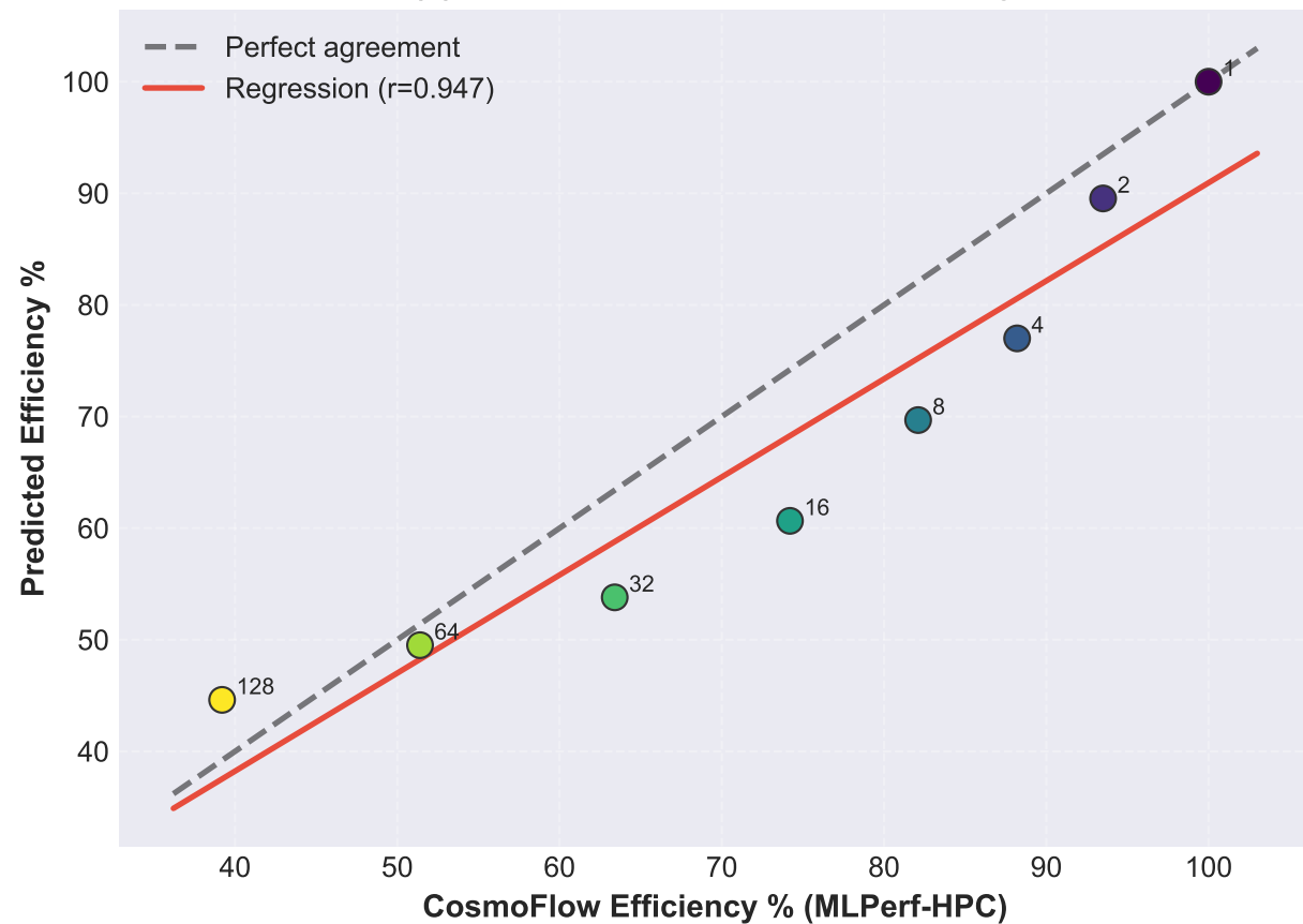
(a) Predicted vs. Measured Efficiency
