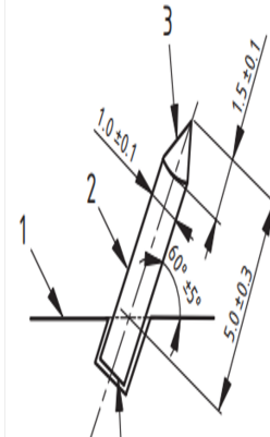
Key 1 Surface of pin bar 2 Pin 3 Pointed end of pin 4 Flat end of pin fitted into blind hole in pin bar c) Detailed view of a pin
