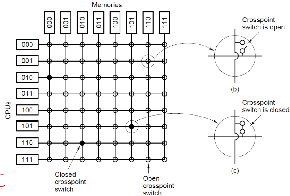
Crossbar connection
