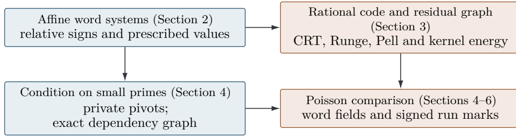
Figure 1: The arithmetic and probabilistic interfaces. The weighted two-window estimate bounds the separated-pair term. Private pivots supply the exact conditional graph and the correct marginals; local overlap is treated separately. Neither interface is dispensable.
