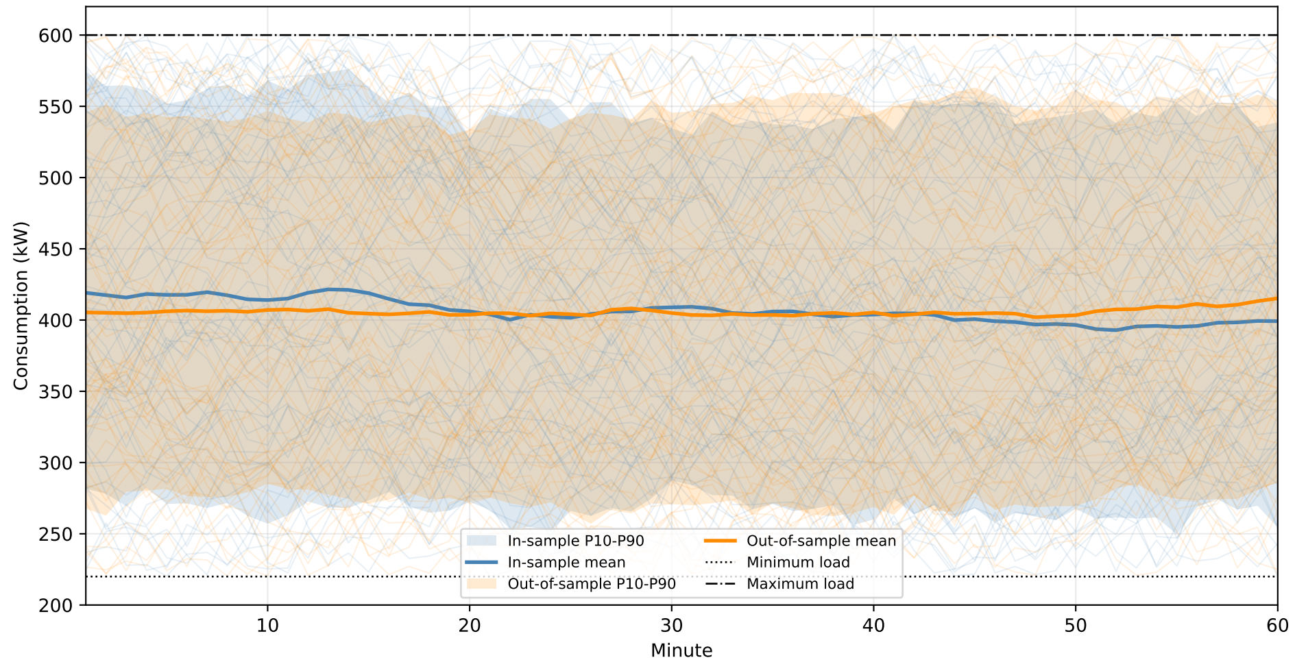
Generated Load Profiles
