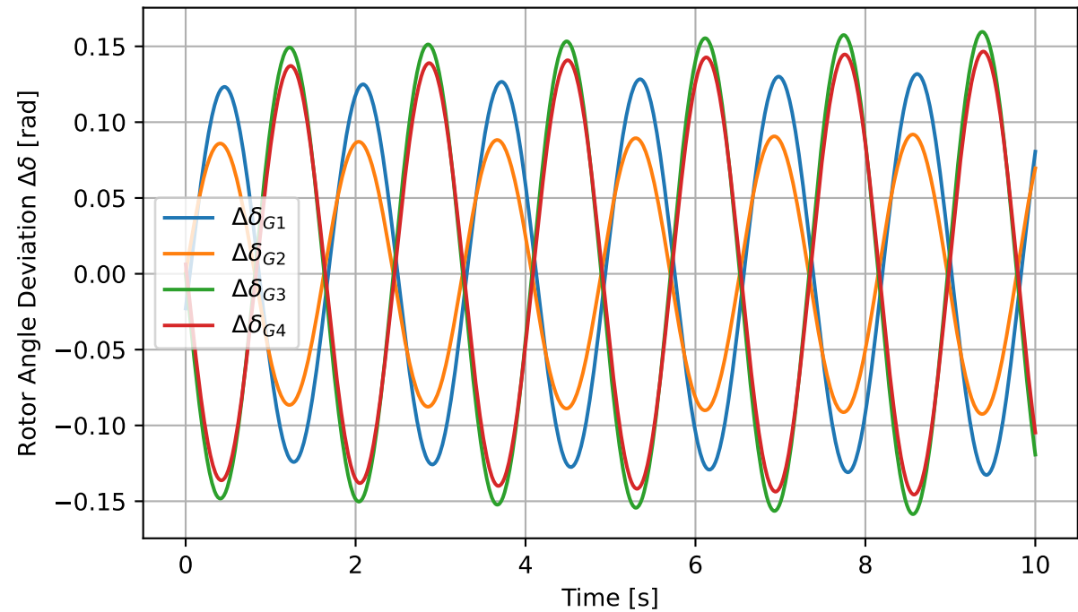
Time Response - Inter-Area Mode Excitation
