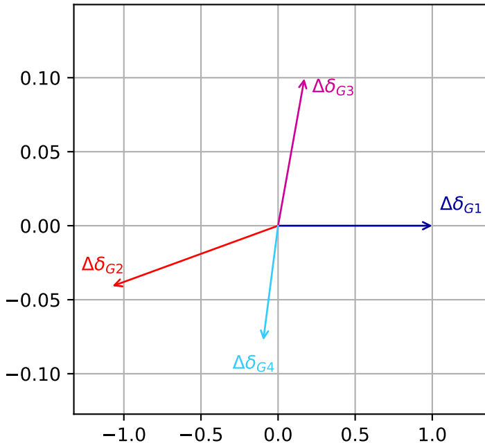
Mode Shape for Mode lambda_17
