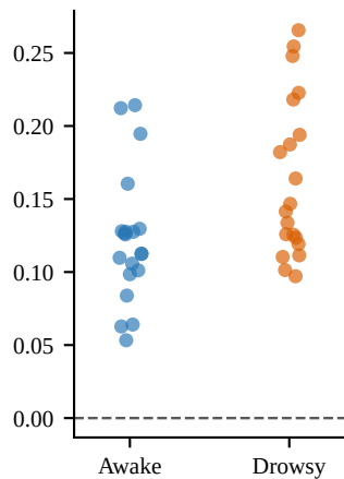
(E) LAM
