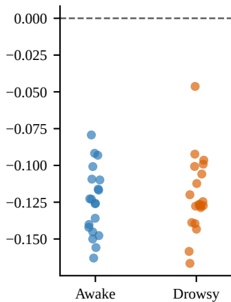
(E) LAM
