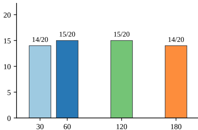
(C) DET ( \Delta < 0 )
