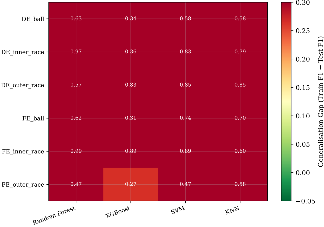
Fig. 8a: Per-Class Severity Generalisation Gap (Train: 0.007" + 0.014", Test: 0.021")
