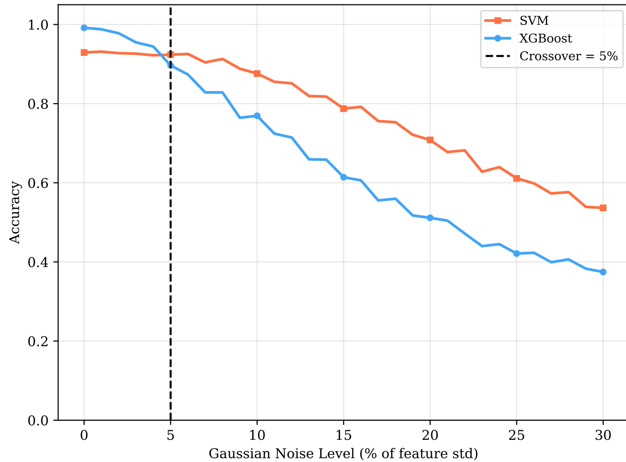
Fig. 8b: SVM vs XGBoost Noise Robustness (Crossover Threshold Detection)
