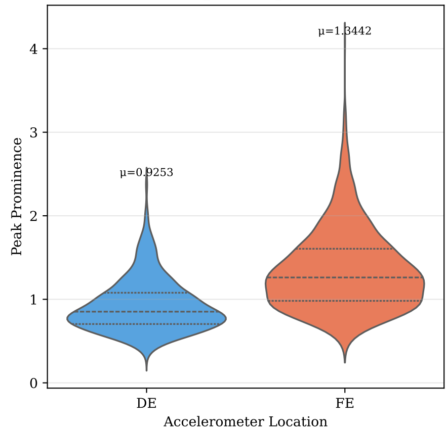
Fig. 9: Spectral Peak Prominence at BSF (DE_ball vs FE_ball)
