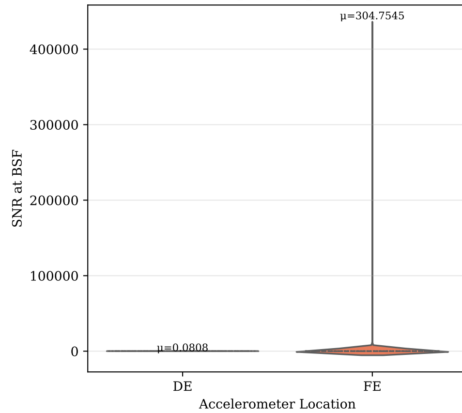
Fig. 9: SNR at Ball Spin Frequency (DE_ball vs FE_ball)
