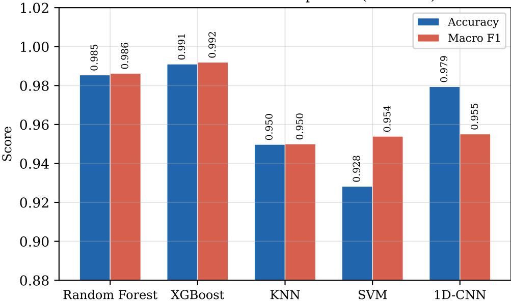
Model Performance Comparison (5-fold CV)
